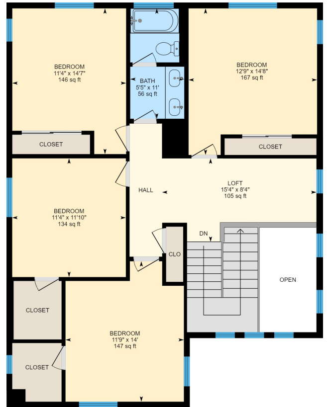
2ND FLOOR
